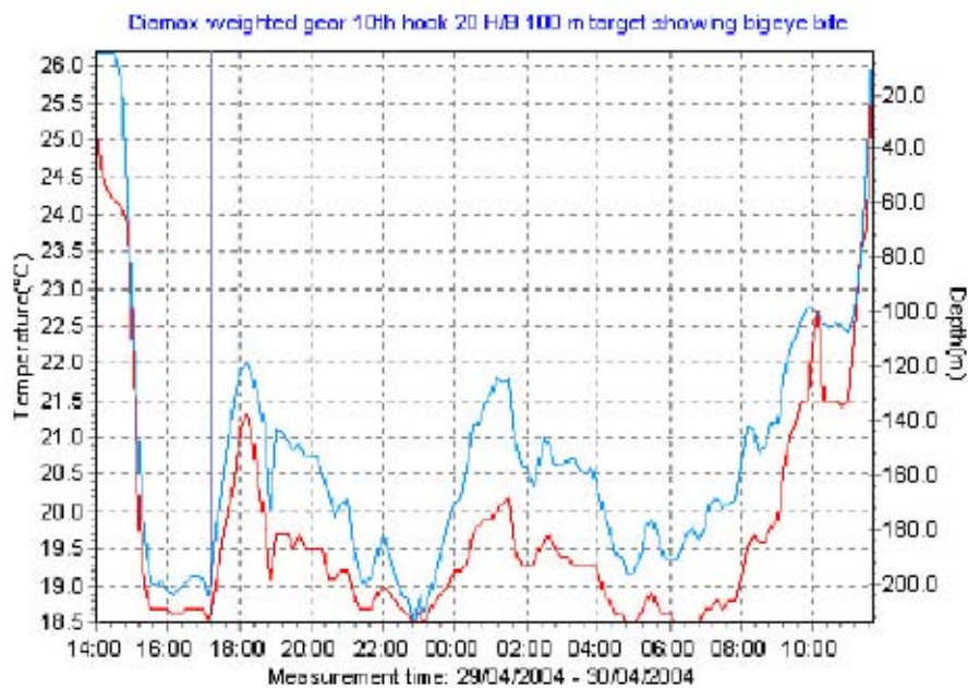
Figure 17: Temperature/depth graph for 10th hook in a weighted basket of 20 hooks and a target depth for shallowest hook of 100 m. The spike at 17:15 indicates a bigeye tuna bite. Depth was 200 m and temperature was 18.5°C. Blue line (upper) is depth, red line (lower) is temperature.
