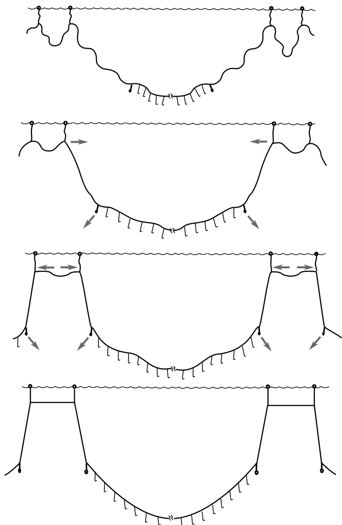
Figure 4: Settling sequence of weighted longline.
