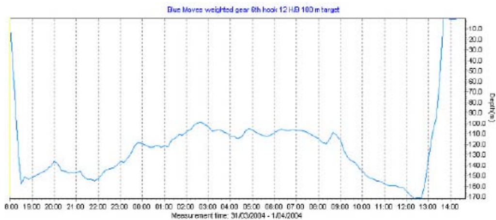
Figure 7: Depth graph for 6th hook in a 12 hook basket using lead weights with a target depth for the shallowest hook of 100 m using the line setter. SR was 0.75. Average depth of hook was about 140 metres.
