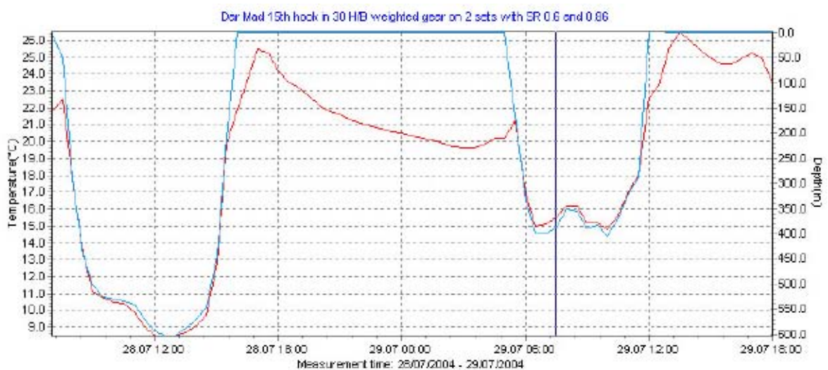
Figure 20: Temperature/depth graph for two sets on F/V Dar Mad. Left side is for deepest hook in a 30 hook basket with target depth of 140 m for shallowest hook and SR of 0.60 on 28 July. Right side is deepest hook in a 30 hook basket with target depth of 120 m for shallowest hook and SR of 0.86 on 29 July. Upper line (blue) is depth, lower line (red) is temperature. The vertical line indicates a probable bigeye tuna bite at 07:30 at a depth of 388 metres and a temperature of 15.5°C.
