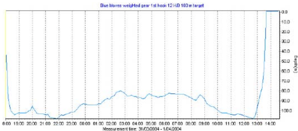
Figure 6: Depth graph for 1st hook in a 12 hook basket using lead weights with a target depth for the shallowest hook of 100 m using the line setter. SR was 0.75. Average depth of hook was about 95 metres.
