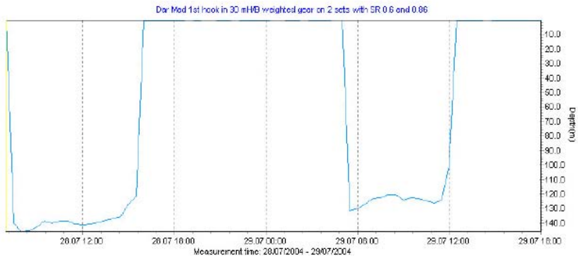
Figure 19: Depth graph for two sets on F/V Dar Mad. Left side is for the shallowest hook in a 30 hook basket with target depth of 140 m for the shallowest hook and an SR of 0.60 on 28 July. Right side is for the shallowest hook in a 30 hook basket with target depth of 120 m for the shallowest hook and SR of 0.86 on 29 July.
